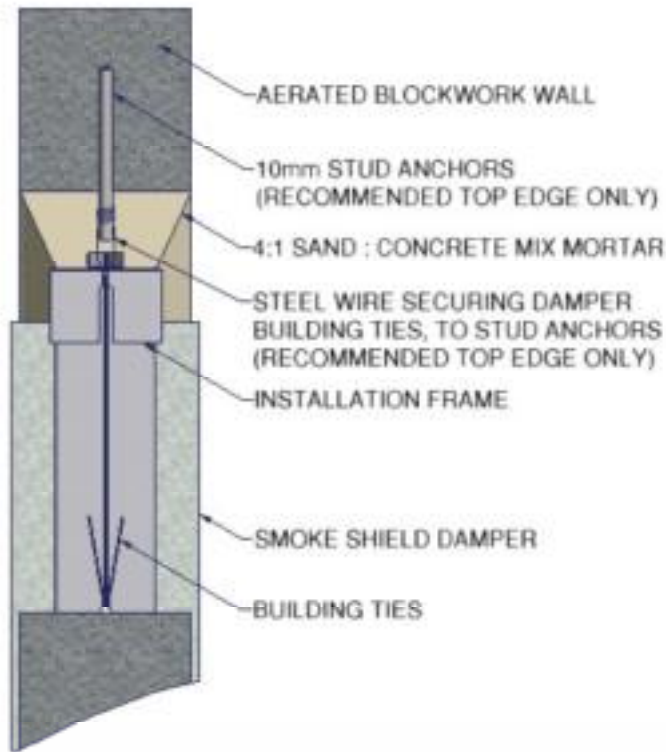
VIEW A (ALL ROUND DETAIL)
